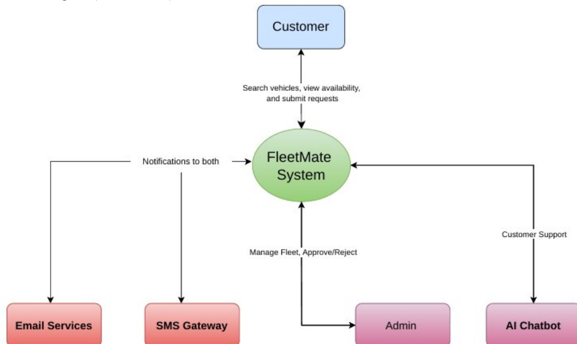
Data Flow Diagram (DFD-Level 0)
